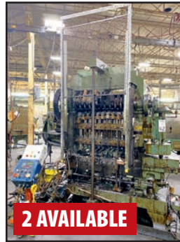
WATERBURY FARREL 2010 EYELET PRESSES
