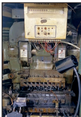
MINSTER PIECE-MAKER P2-45-36 SSDC PRESSES
